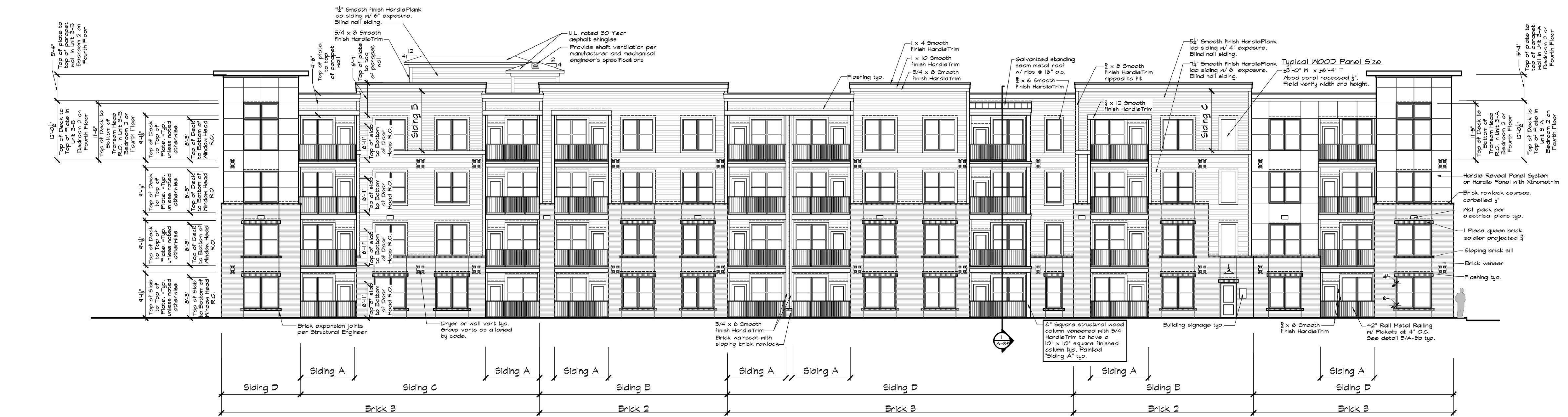
1 BUILDING TYPE I - EXAMPLE ELEVATION - FRONT Scale: 1/8" = 1'-0"
