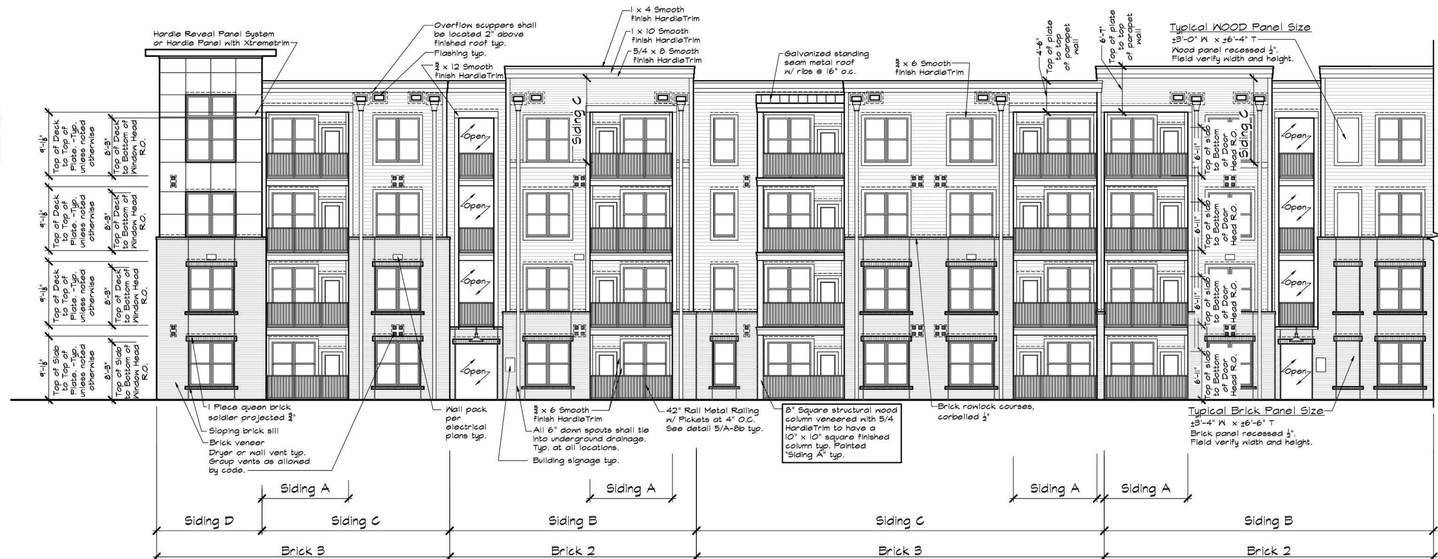
3 BUILDING TYPE II - EXAMPLE ELEVATION - REAR Scale: \frac{1}{8}'' = 1'-0''
