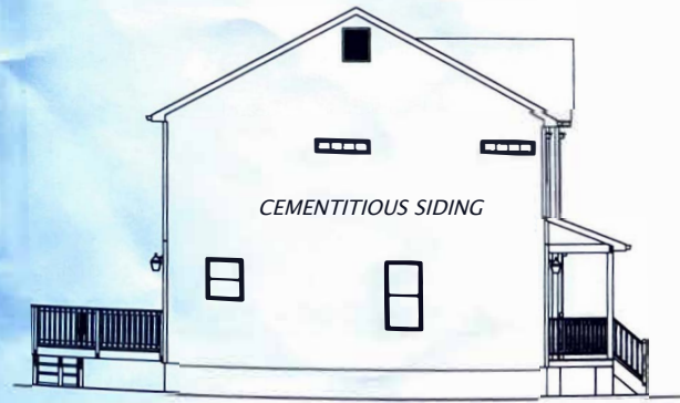
LEFT ELEVATION SCALE: 3/32" = 1'-0"
