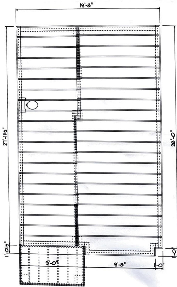
FIRST FLOOR JOIST PLAN SCALE: 3/16" = 1'-0"
