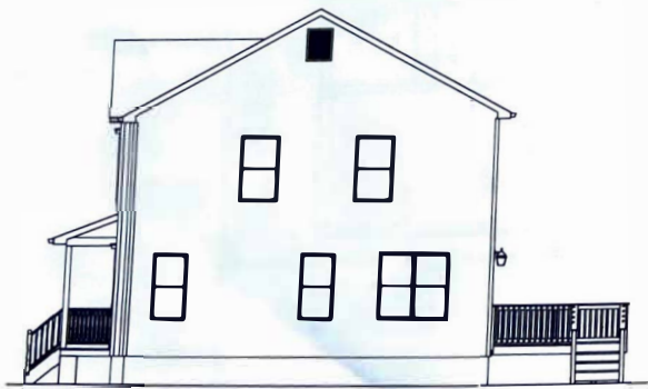
RIGHT ELEVATION SCALE: 3/32" = 1'-0"
