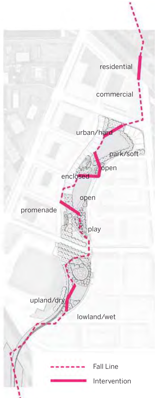
Diamond District Tectonics
