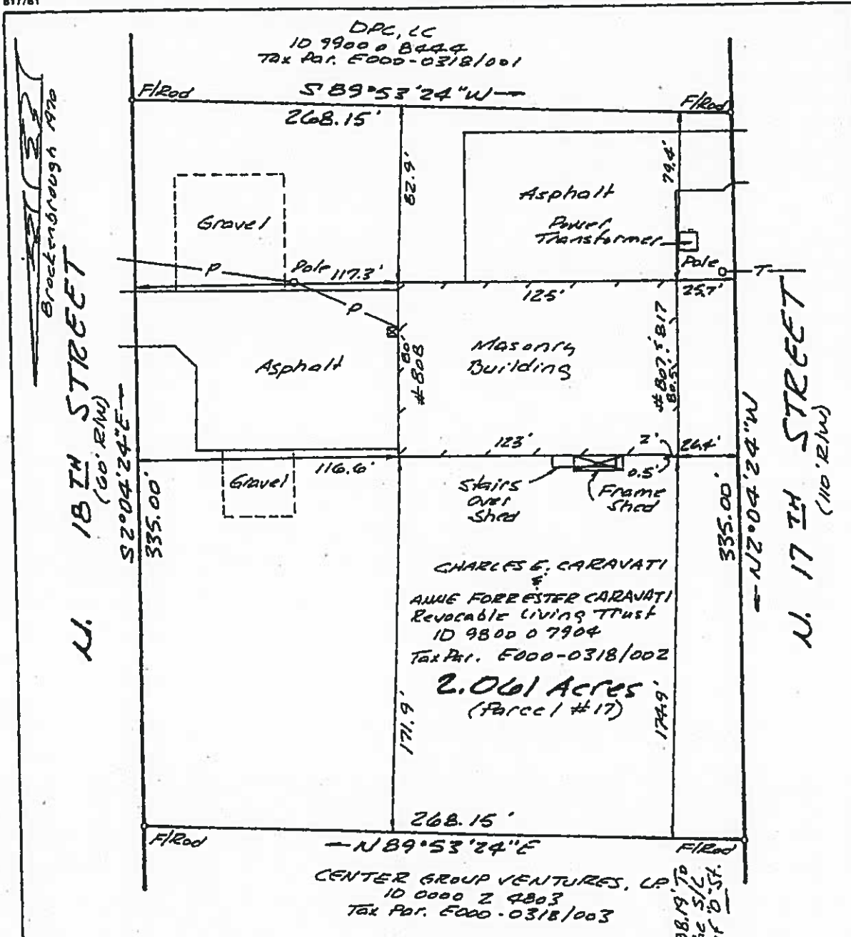
Physical Survey Map Showing 2.061 Acres Of Land On N. 17th Street & N. 18th Street In The City Of Richmond, Virginia
