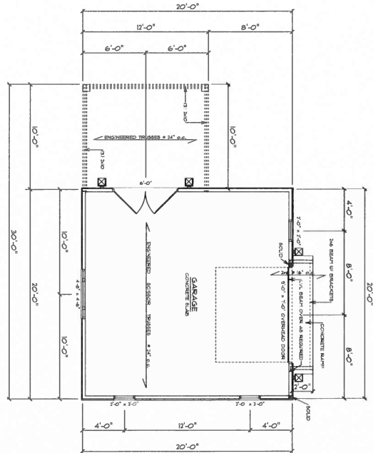
FLOOR PLAN SCALE: 1/4\"/>
