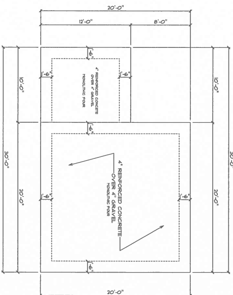
FOUNDATION/SLAB PLAN SCALE: 1/4\"/>
