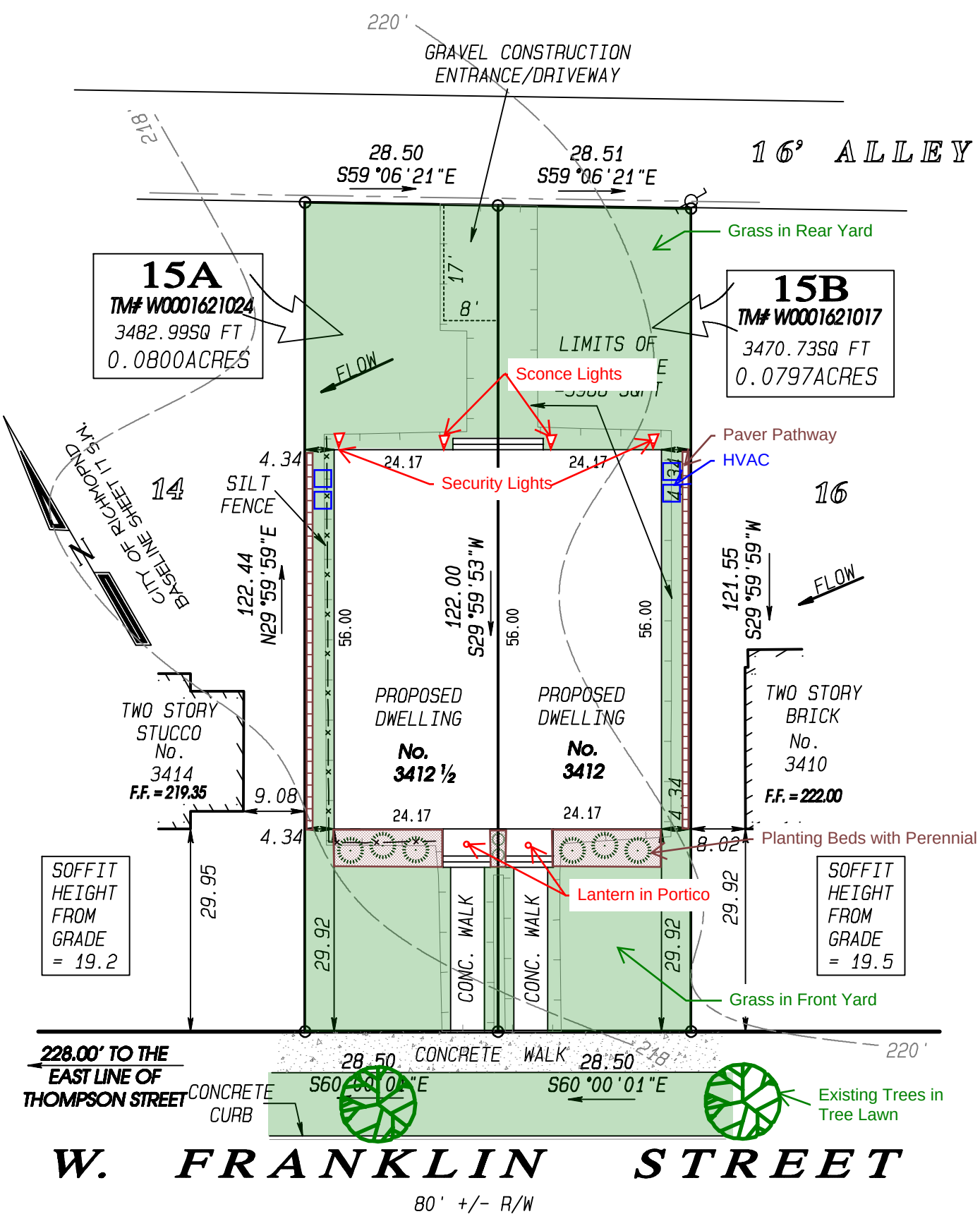
PLOT PLAN SHOWING PROPOSED IMPROVEMENTS ON No. 3412 & No. 3412 1/2 W. FRANKLIN STREET, IN THE CITY OF RICHMOND, VIRGINIA.
