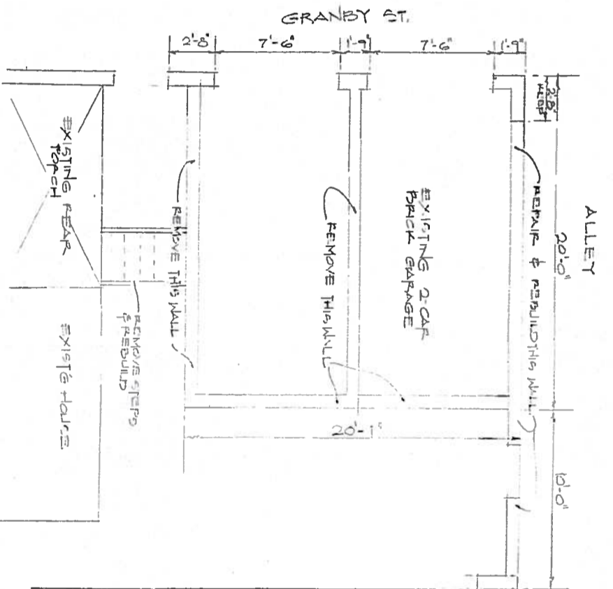
EXISTING GARAGE DEMOLITION PLAN 1/4"=1'-0"
