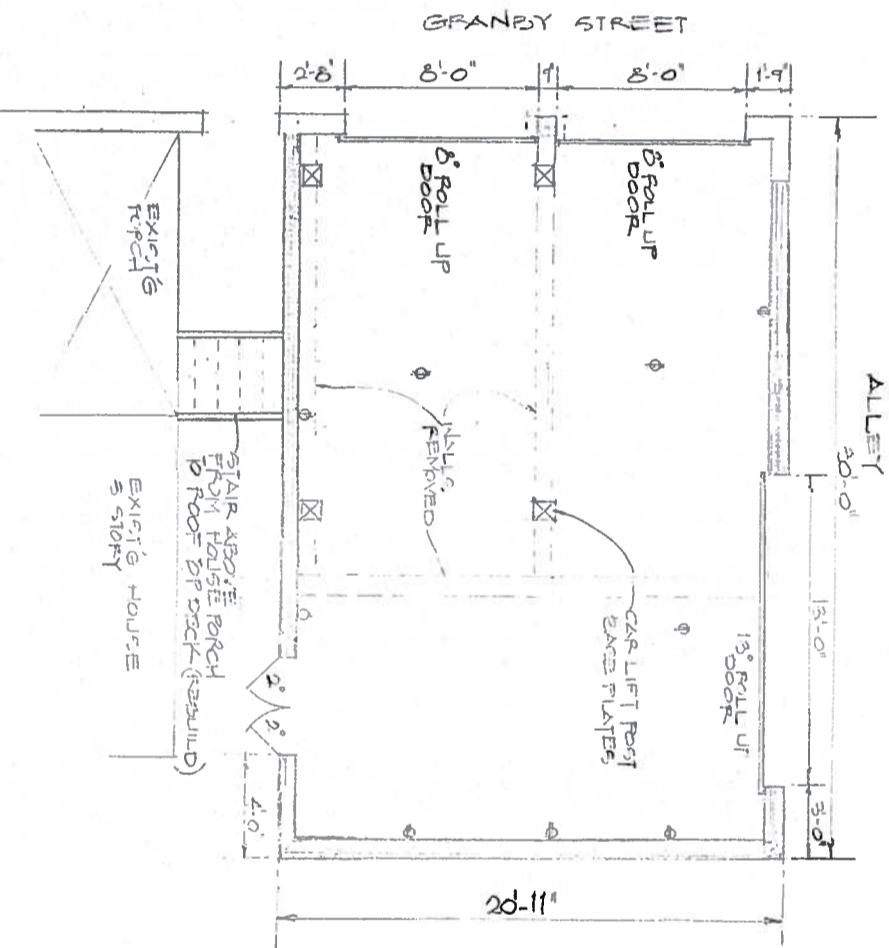
NEW GARAGE PLAN 1/4"=1'-0"
