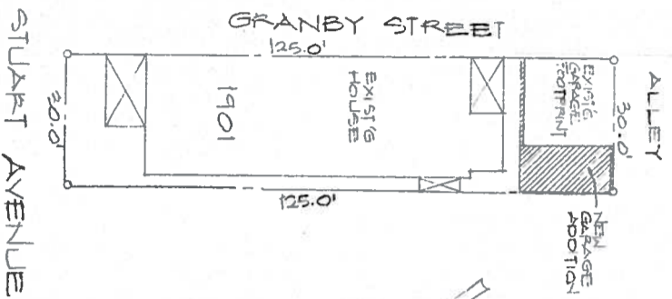
NEW SITE PLAN 1"=20'-0"
