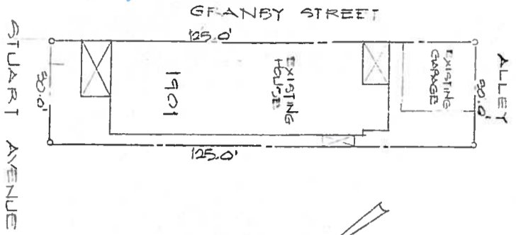
EXISTING SITE PLAN 1"=20'-0"
