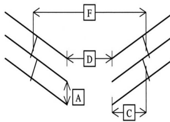
Angled Parking – Interlock to Interlock
