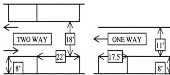
0 Degree - Parallel Parking
