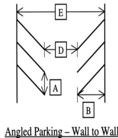
Angled Parking – Wall to Wall
