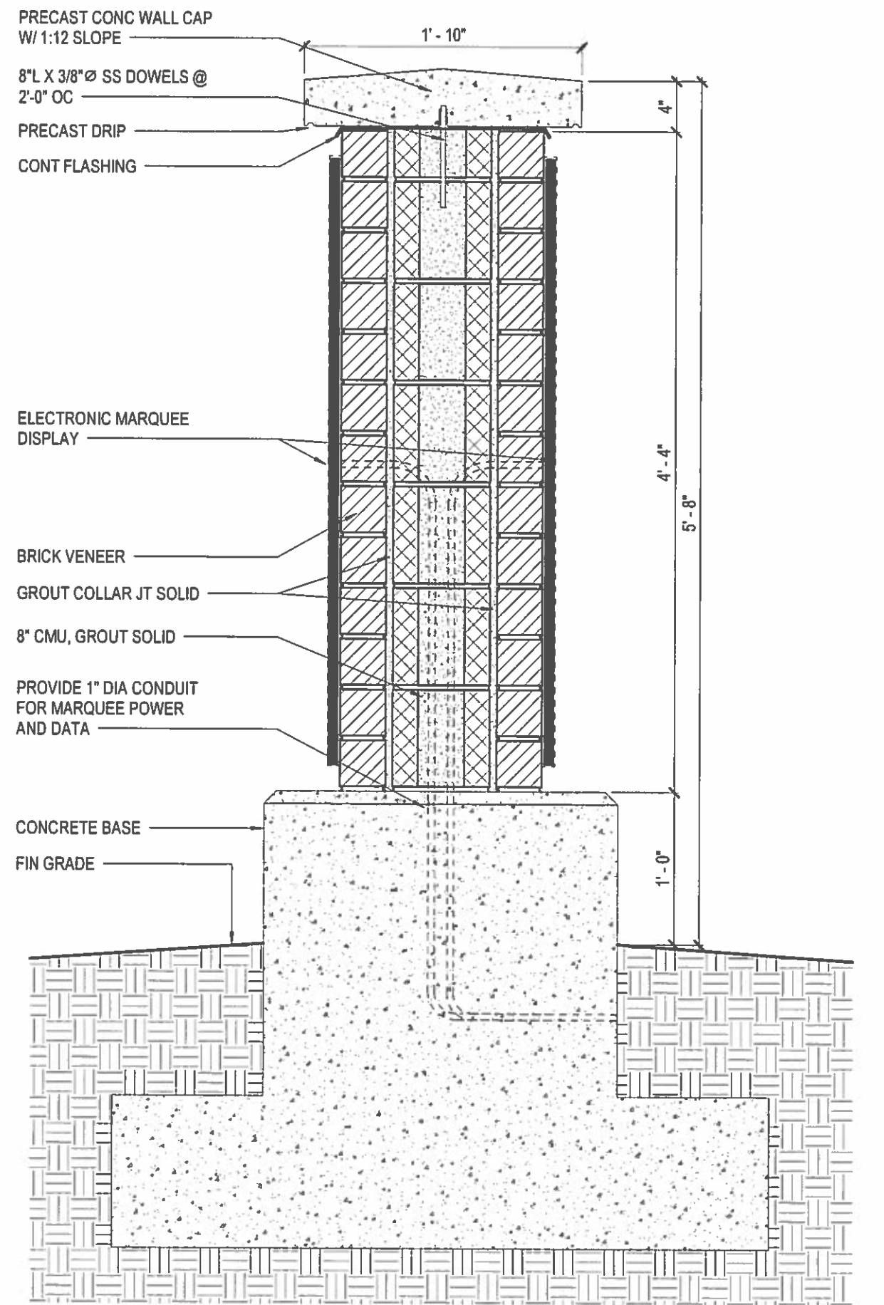
ADDTL MONUMENT SIGN W/ DIGITAL DISPLAY (SECTION)
