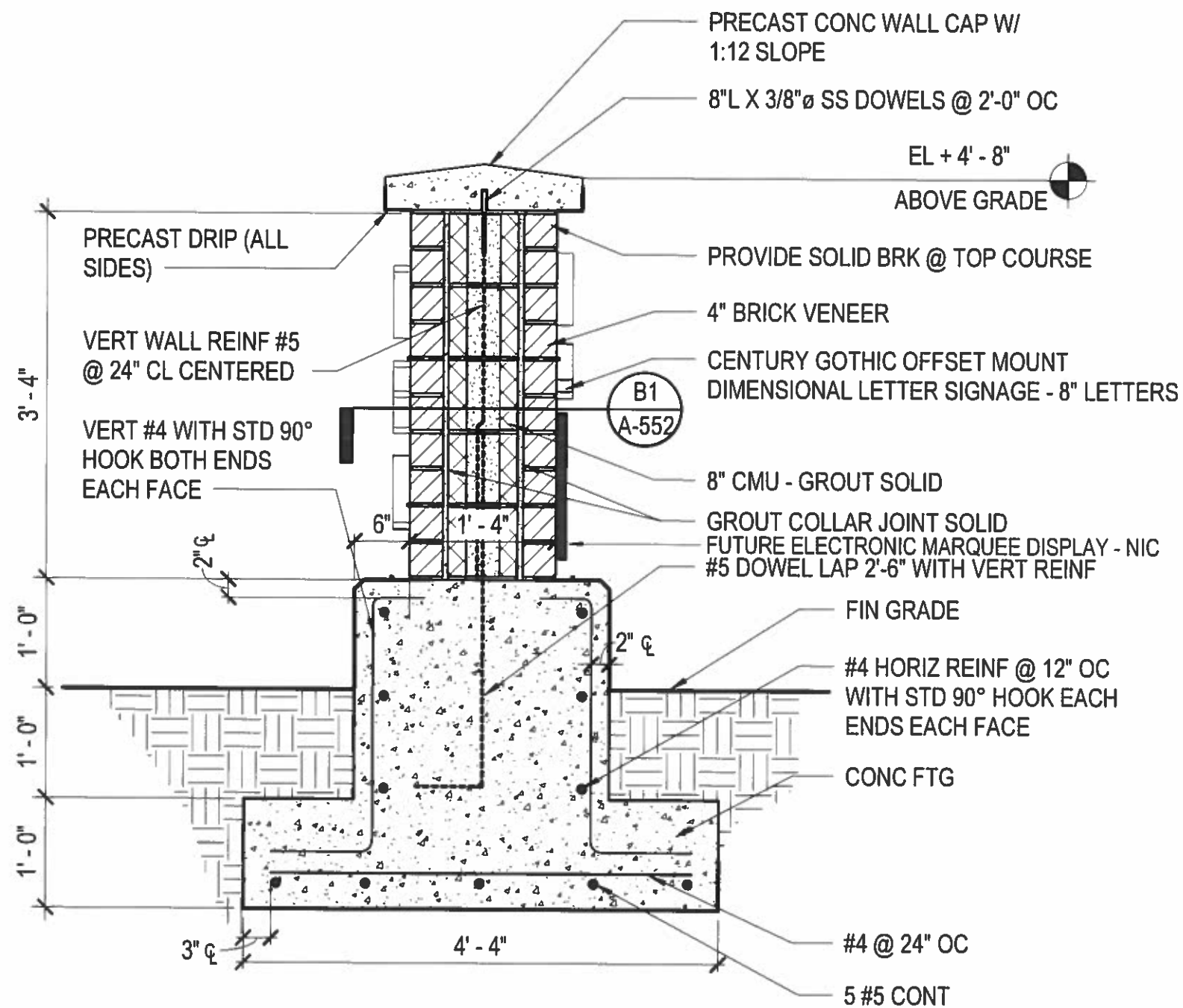
EXISTING MONUMENT SIGN (SECTION)
