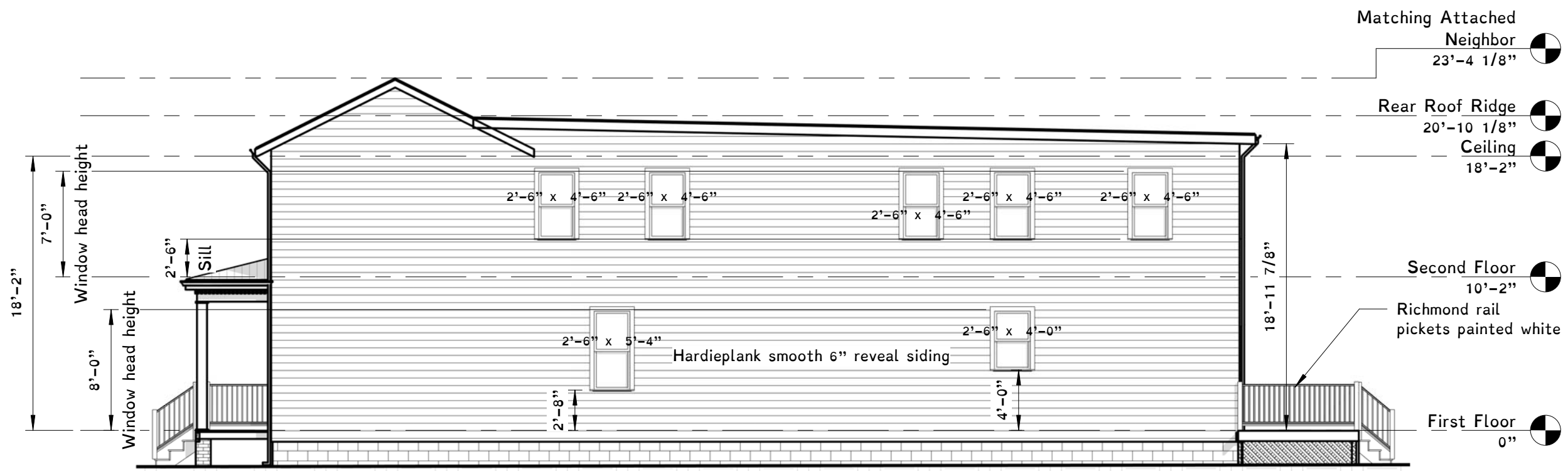
1 North 1/8" = 1'-0"
