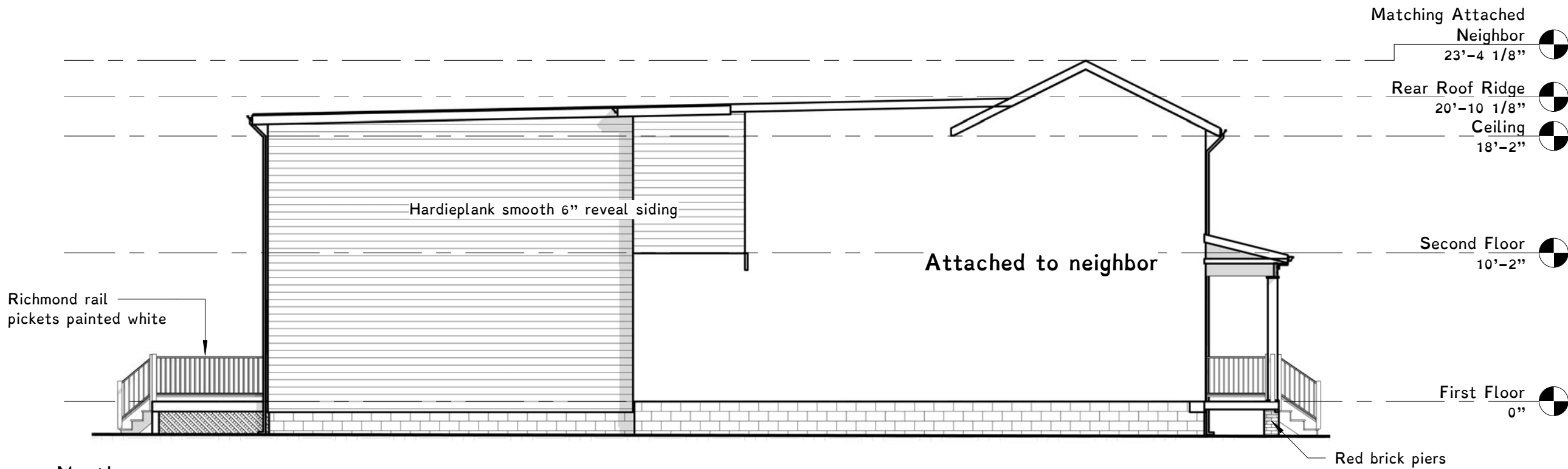
1 North 1/8" = 1'-0"
