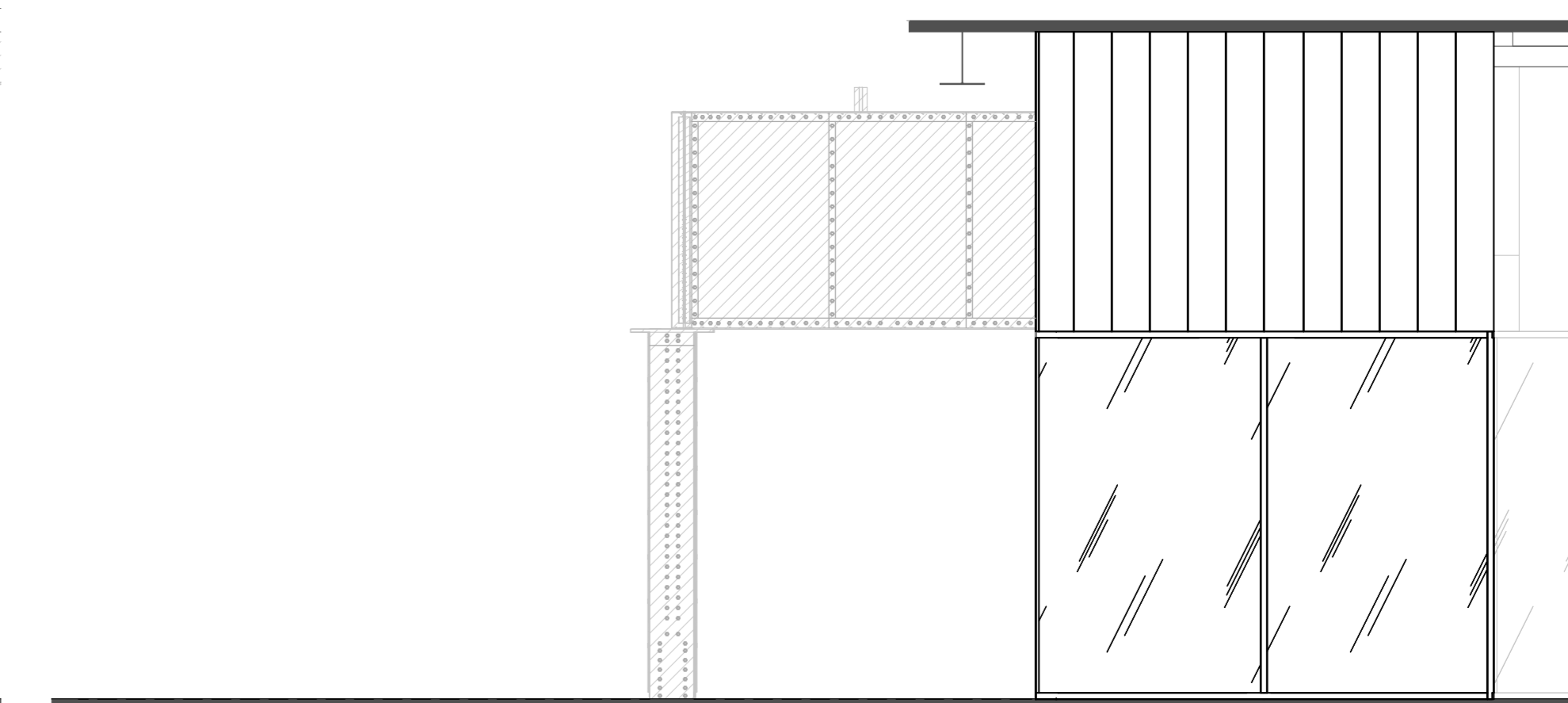
2C ELEVATION - VESTIBULE WEST
