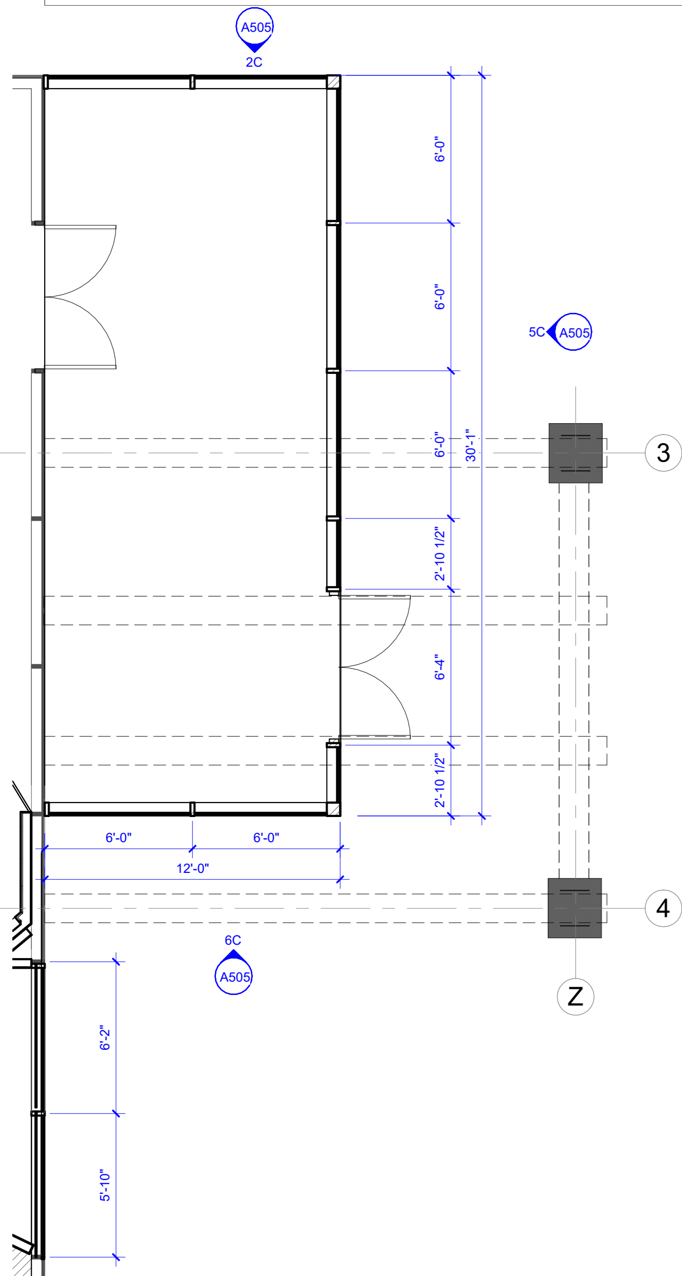
6B ENLARGED PLAN - VESTIBULE
