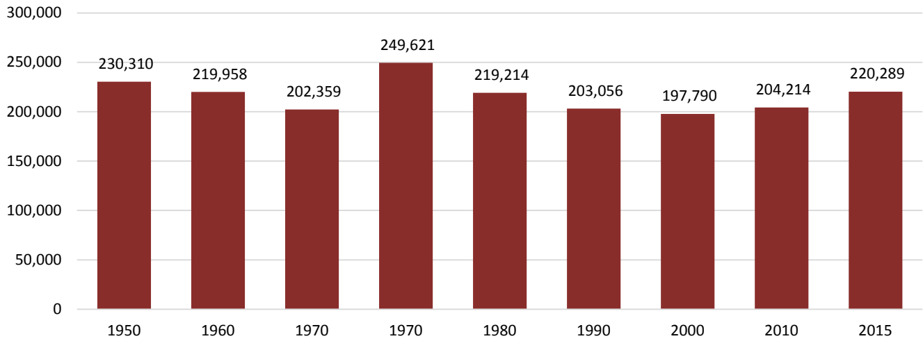
Fig. 2 - Population Change (1950-2015)
