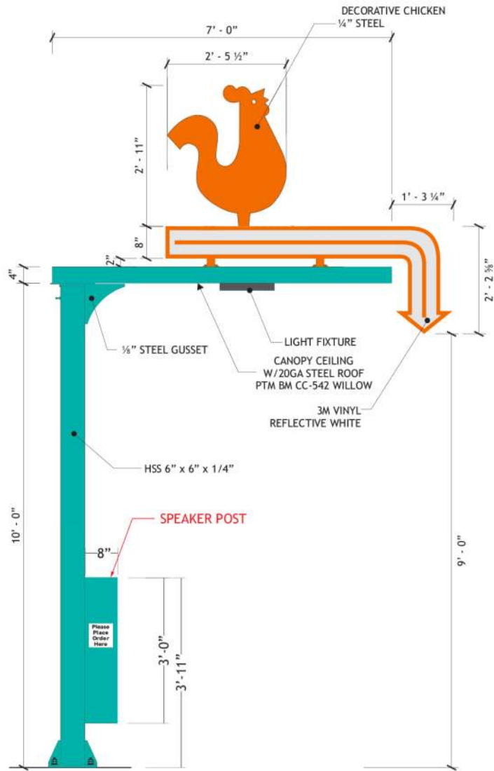
10 SPEAKER POST CANOPY
