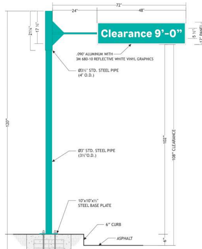
11 CLEARANCE BAR
