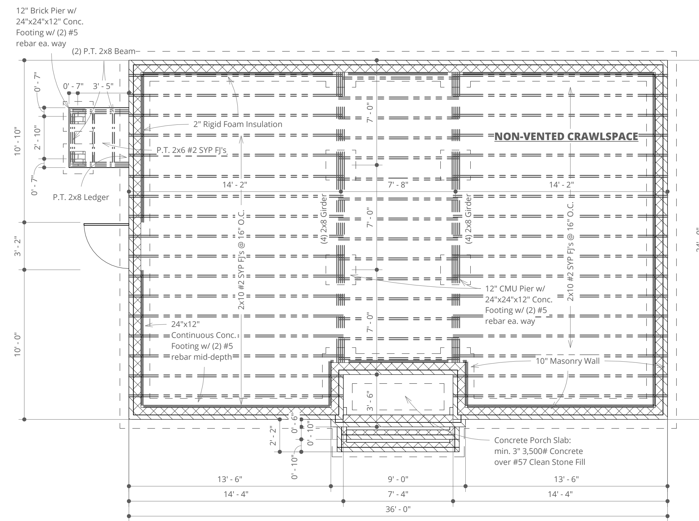
FOOTINGS & FOUNDATION PLAN 1/4" = 1'-0"
