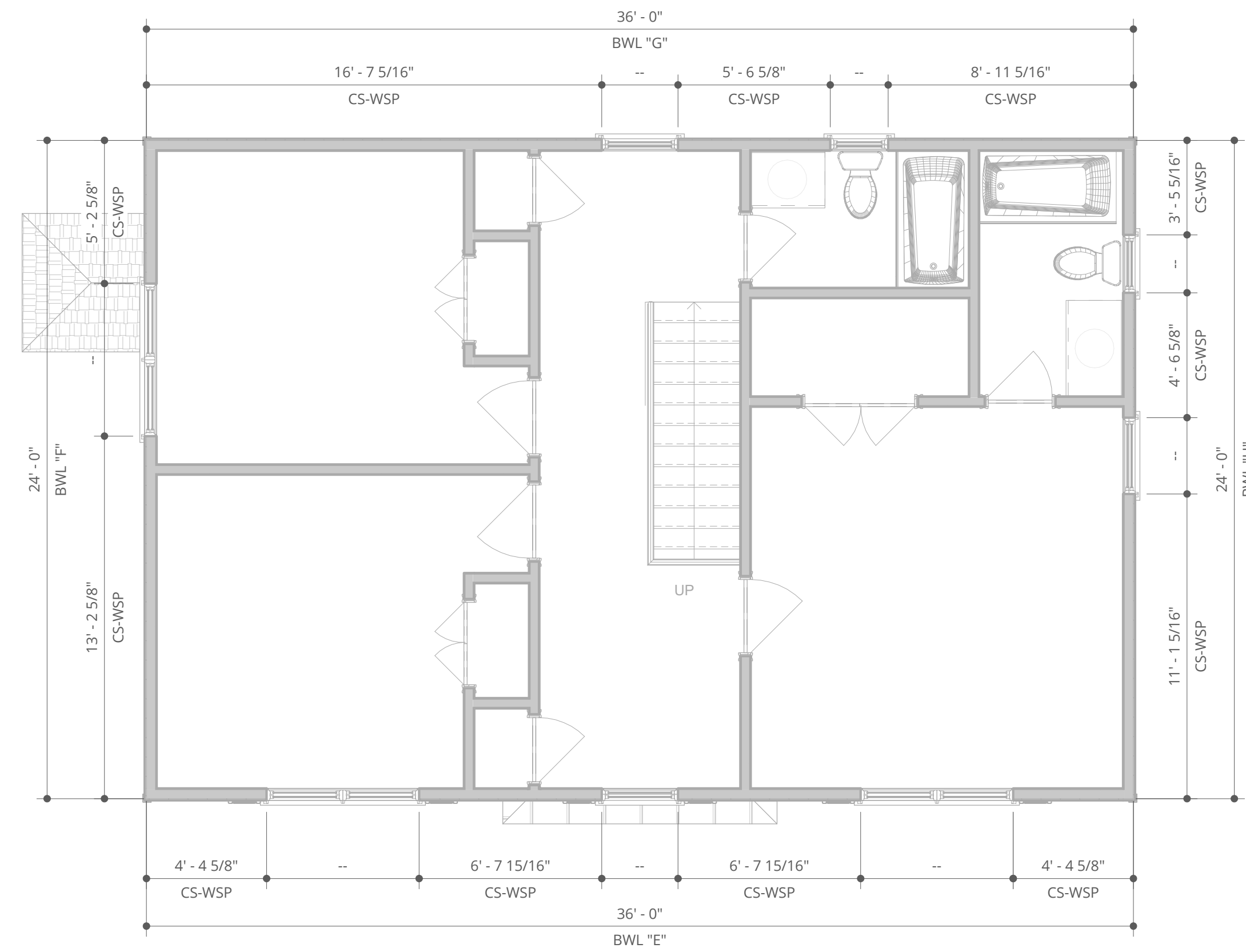
BRACED WALL PLAN -- SECOND FLOOR 1/4" = 1'-0"
