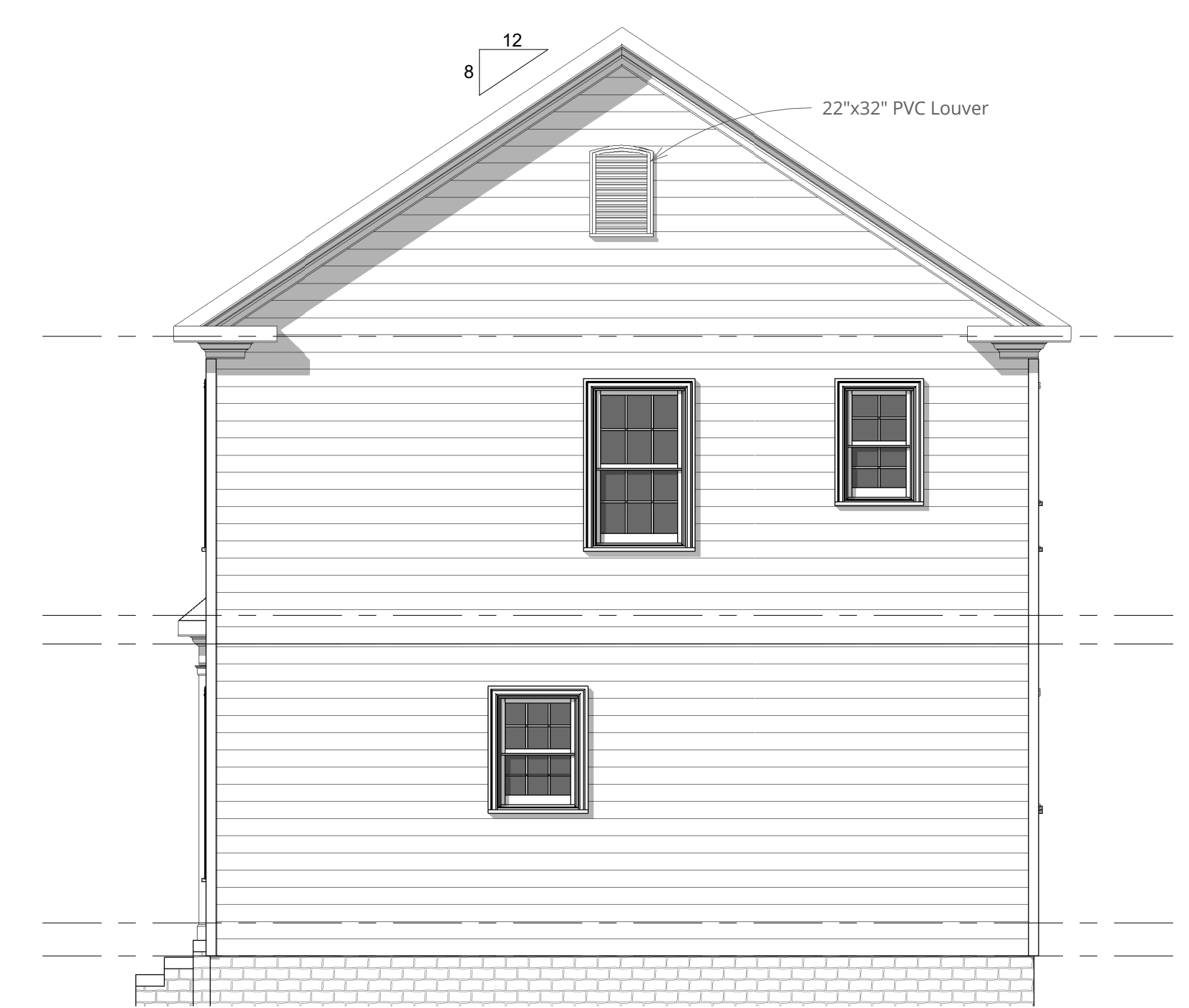
RIGHT ELEVATION 1/4" = 1'-0"
