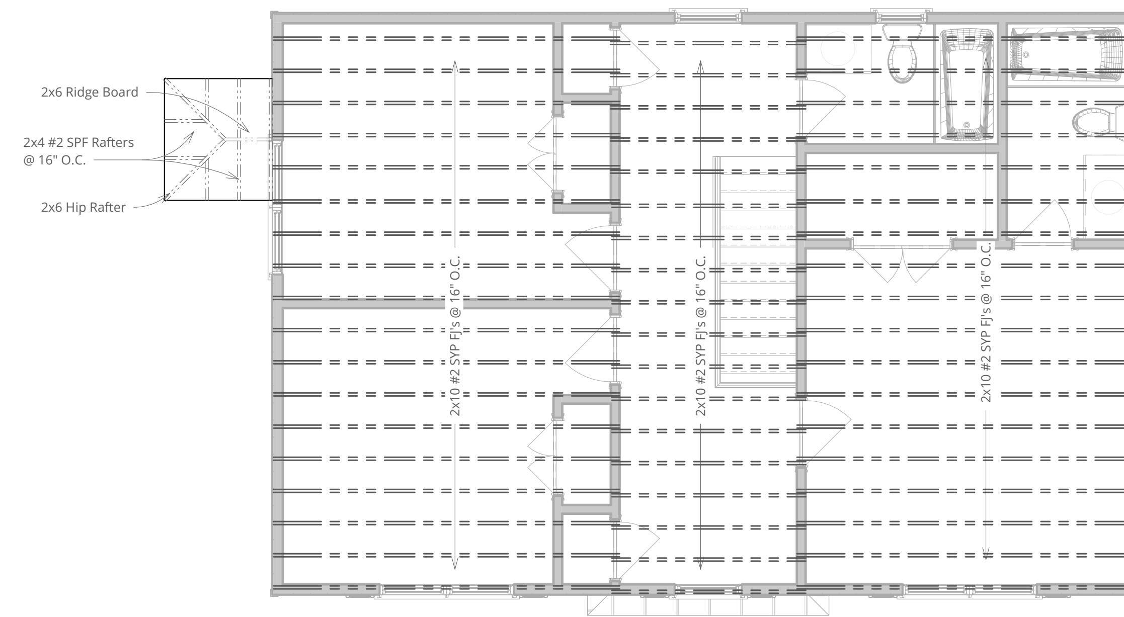
2nd FLOOR CJ FRAMING PLAN 1/4" = 1'-0"
