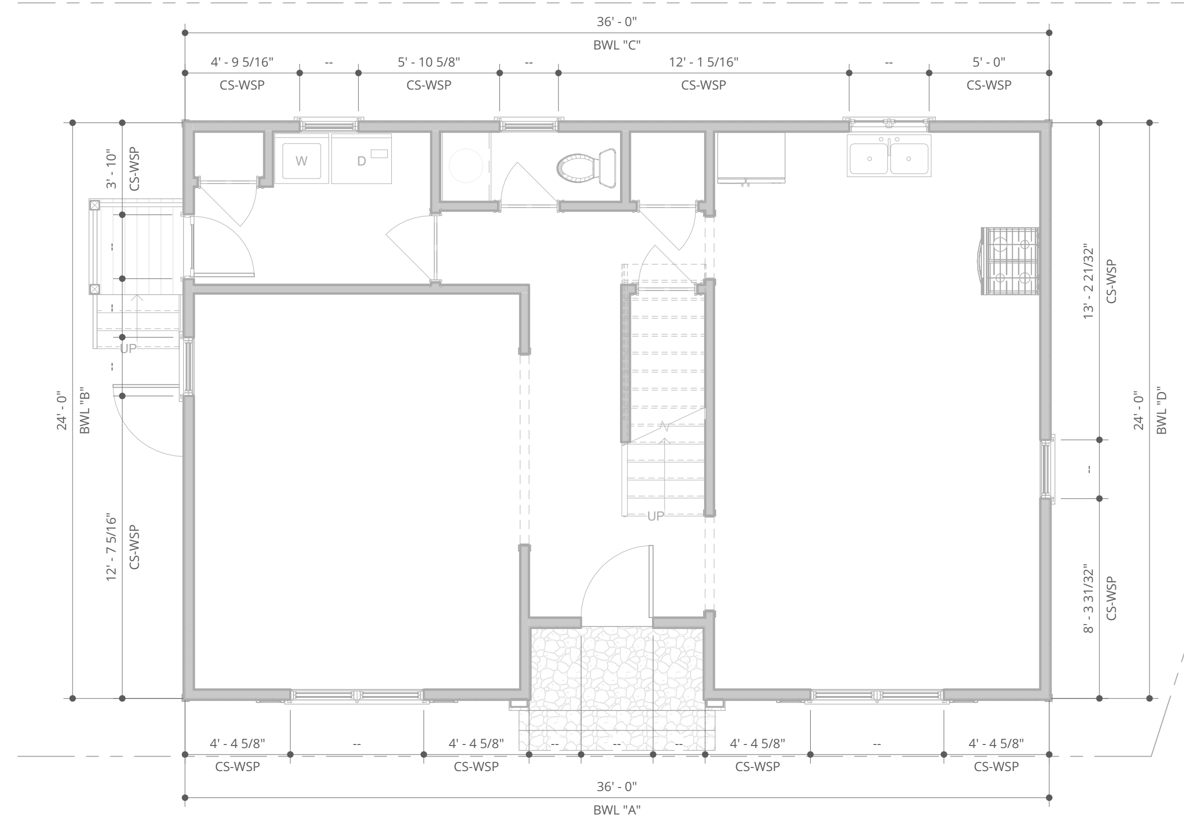
BRACED WALL PLAN -- FIRST FLOOR 1/4" = 1'-0"
