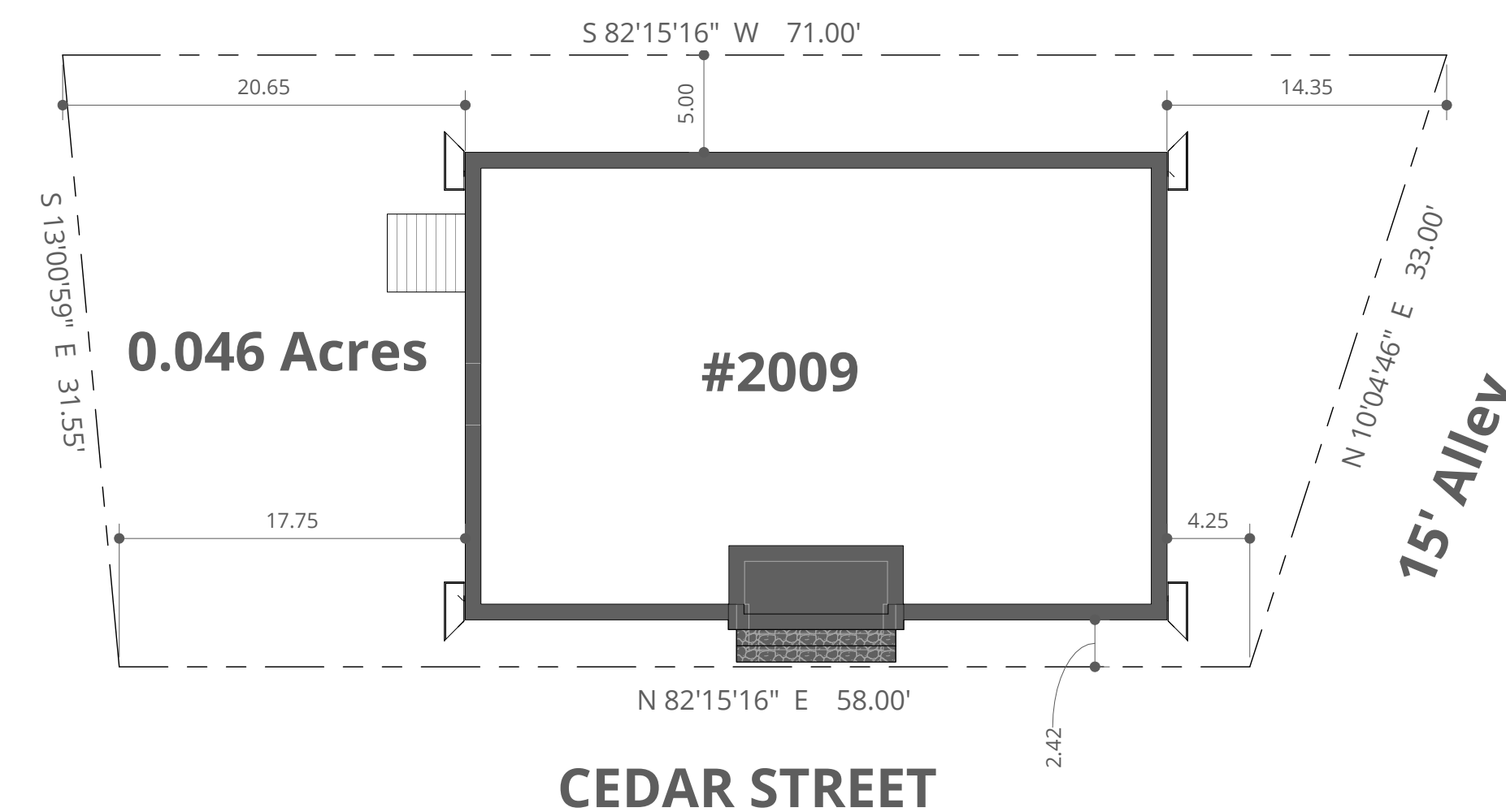
Site Plan 1/8" = 1'-0"
