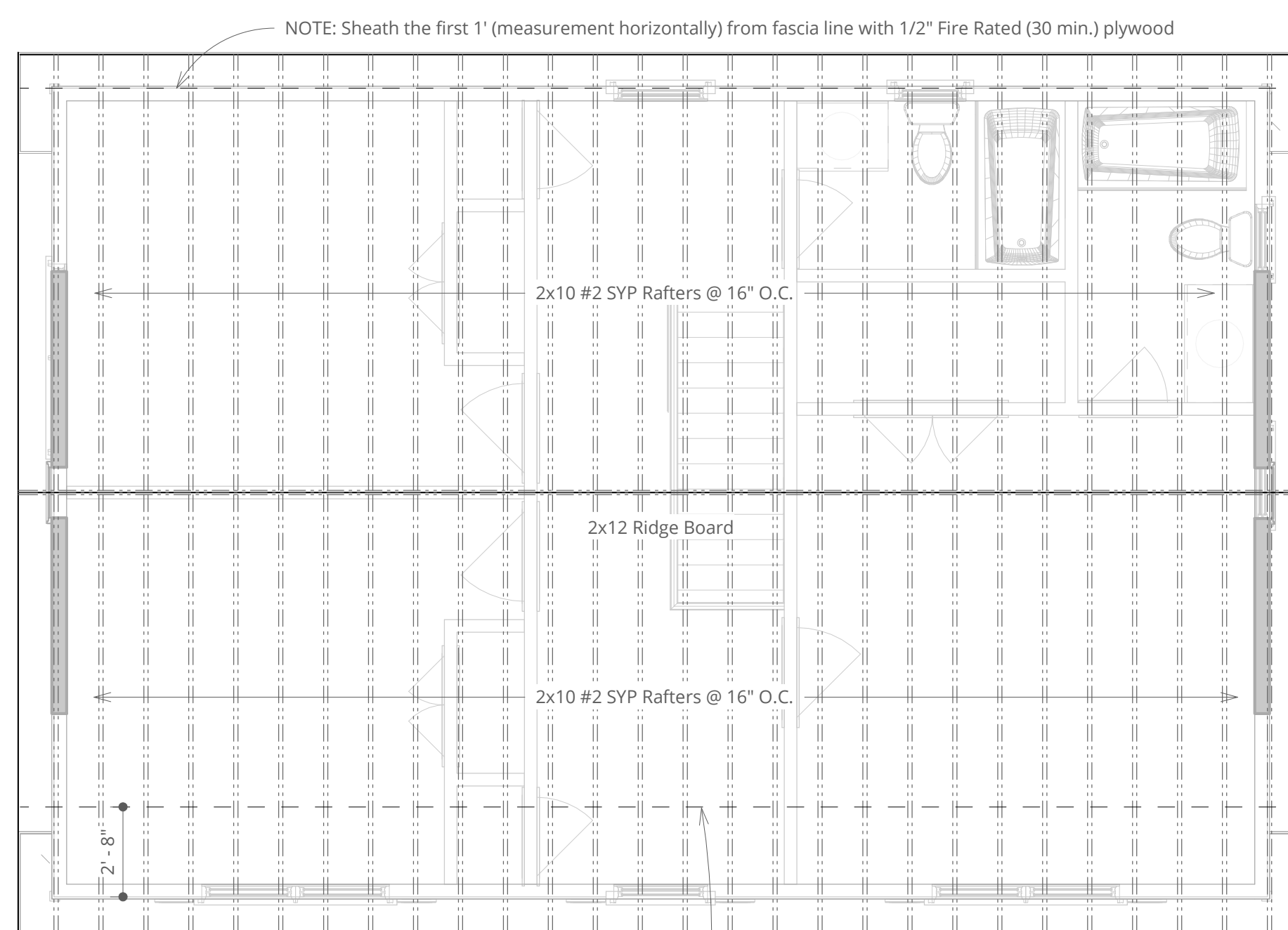
ROOF FRAMING PLAN 1/4" = 1'-0"
