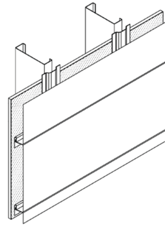
METAL PANEL DETAIL
