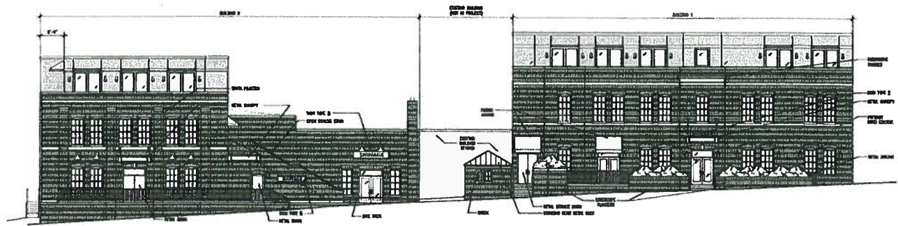
C REAR ELEVATION 1/24/17 1/24/17
