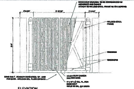
2 ELEVATION DUMPSTER AND COMPACTOR ENCLOSURE SCALE 1/2" = 1'-0"
