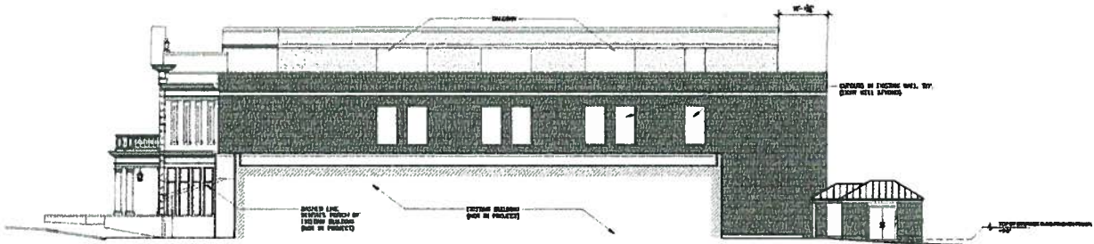
F BUILDING 1 - SIDE ELEVATION SCALE 1/4" = 1'-0"
