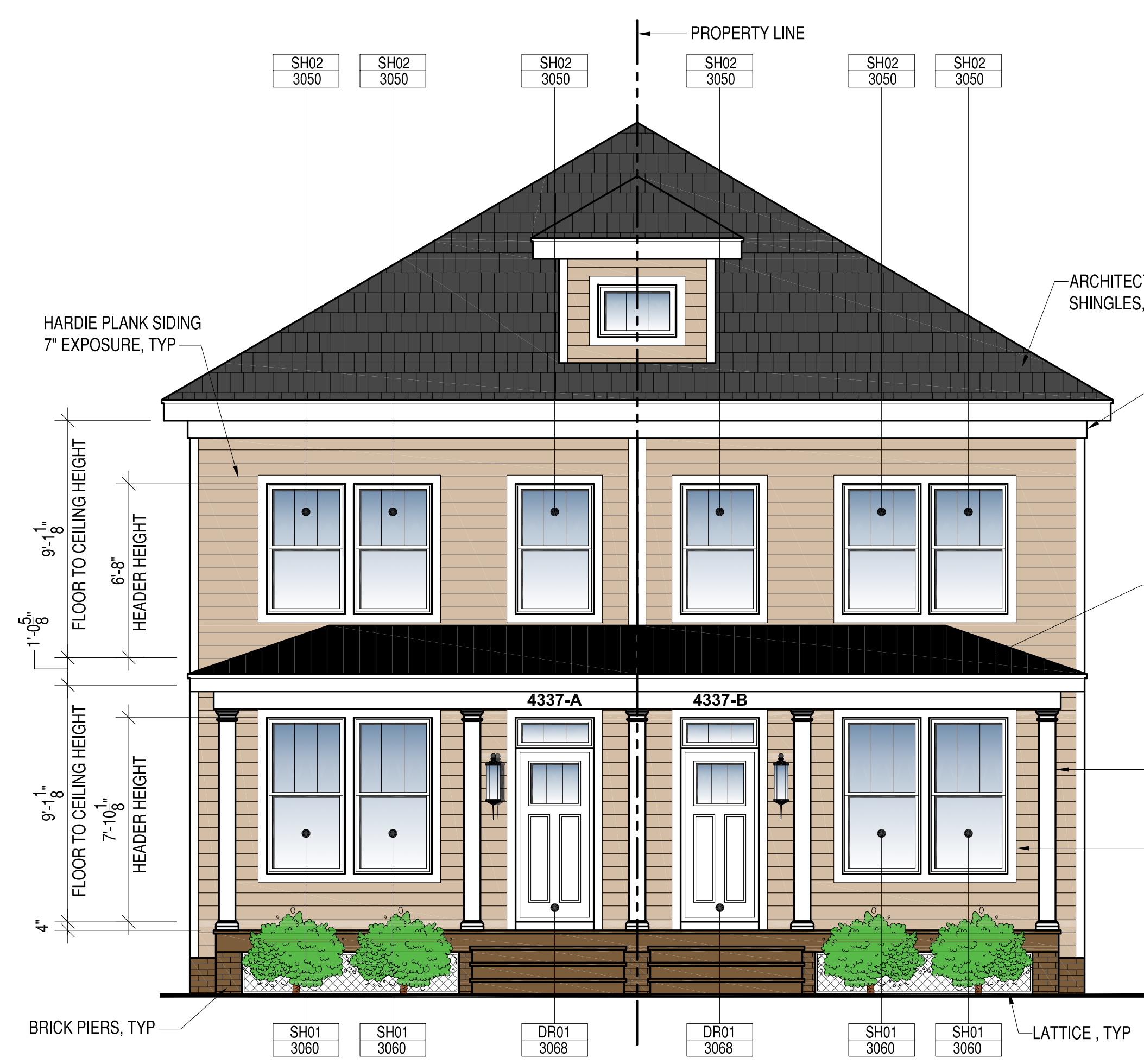
1 PROPOSED FRONT ELEVATION A-201 SCALE: 1/4"=1'-0"
