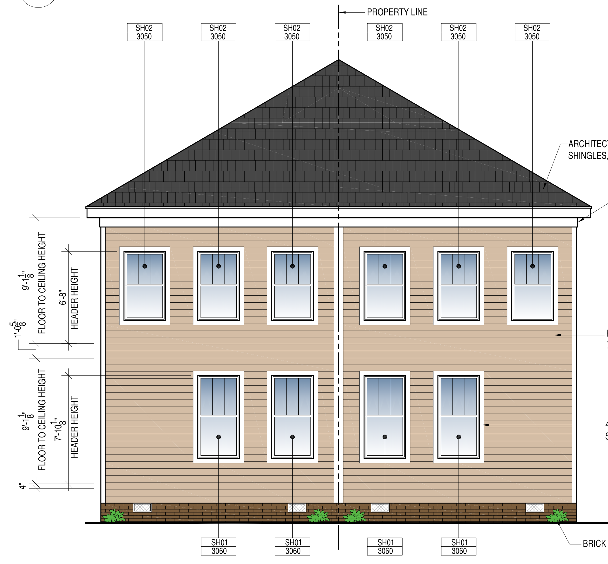
3 PROPOSED REAR ELEVATION A-201 SCALE: 1/4"=1'-0"
