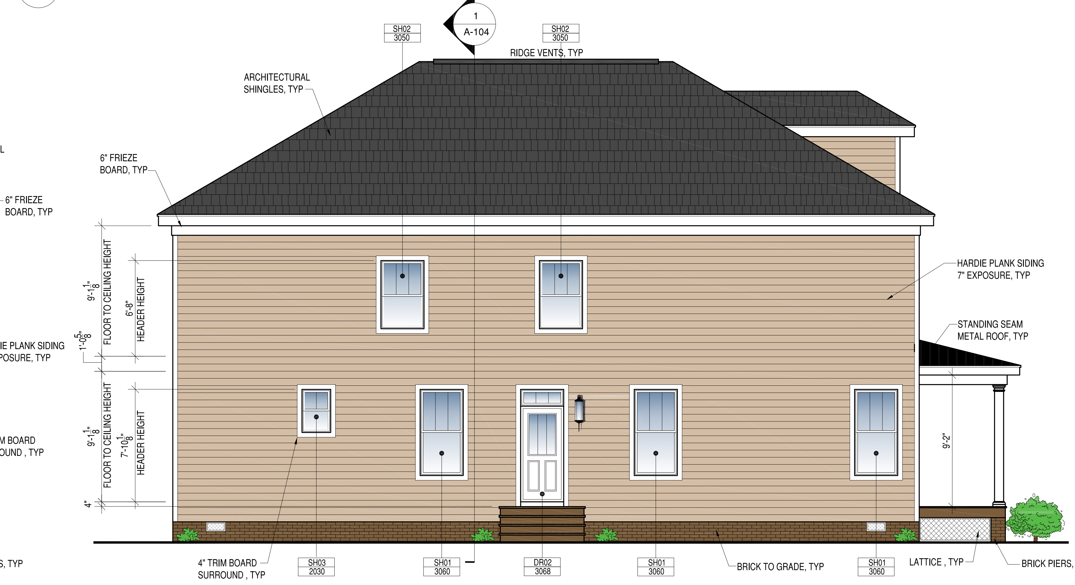
4 PROPOSED LEFT ELEVATION A-201 SCALE: 1/4"=1'-0"
