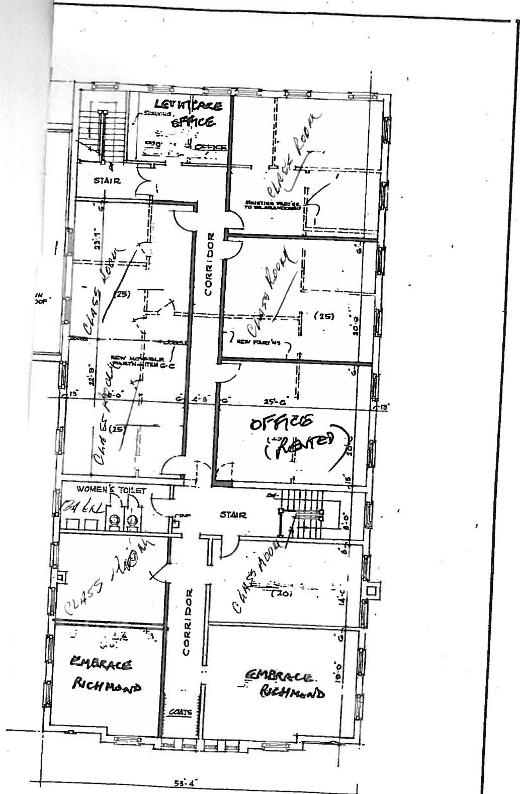
THIRD FLOOR - 1/8" = 1'-0"
