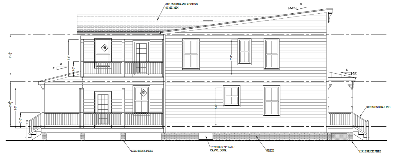
LEFT ELEVATION
