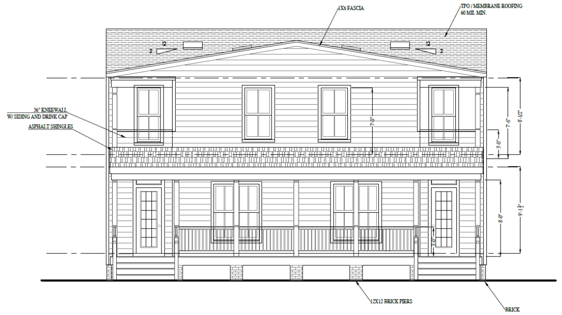
REAR ELEVATION
