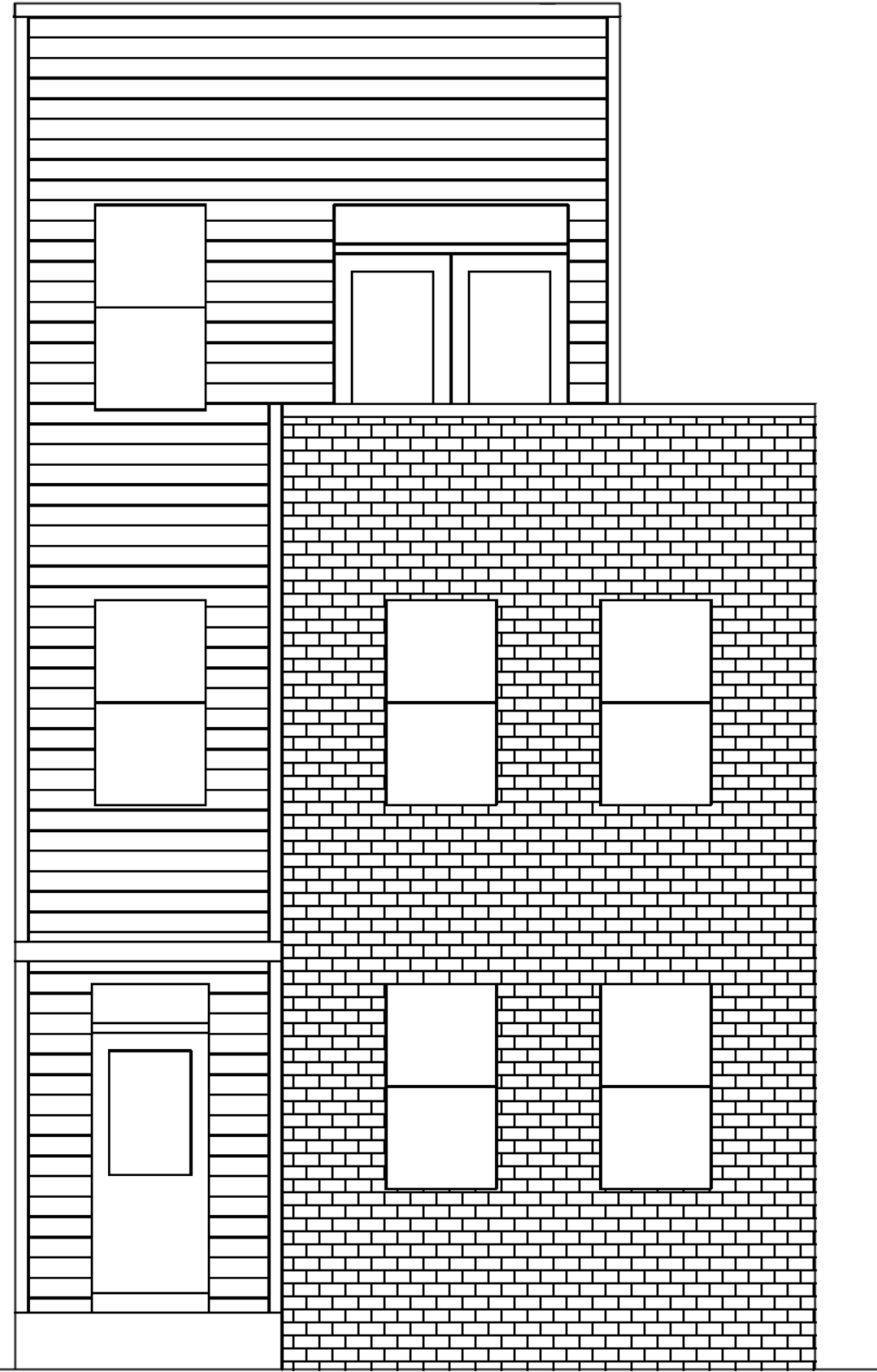
West Elevation 3/8" = 1'
