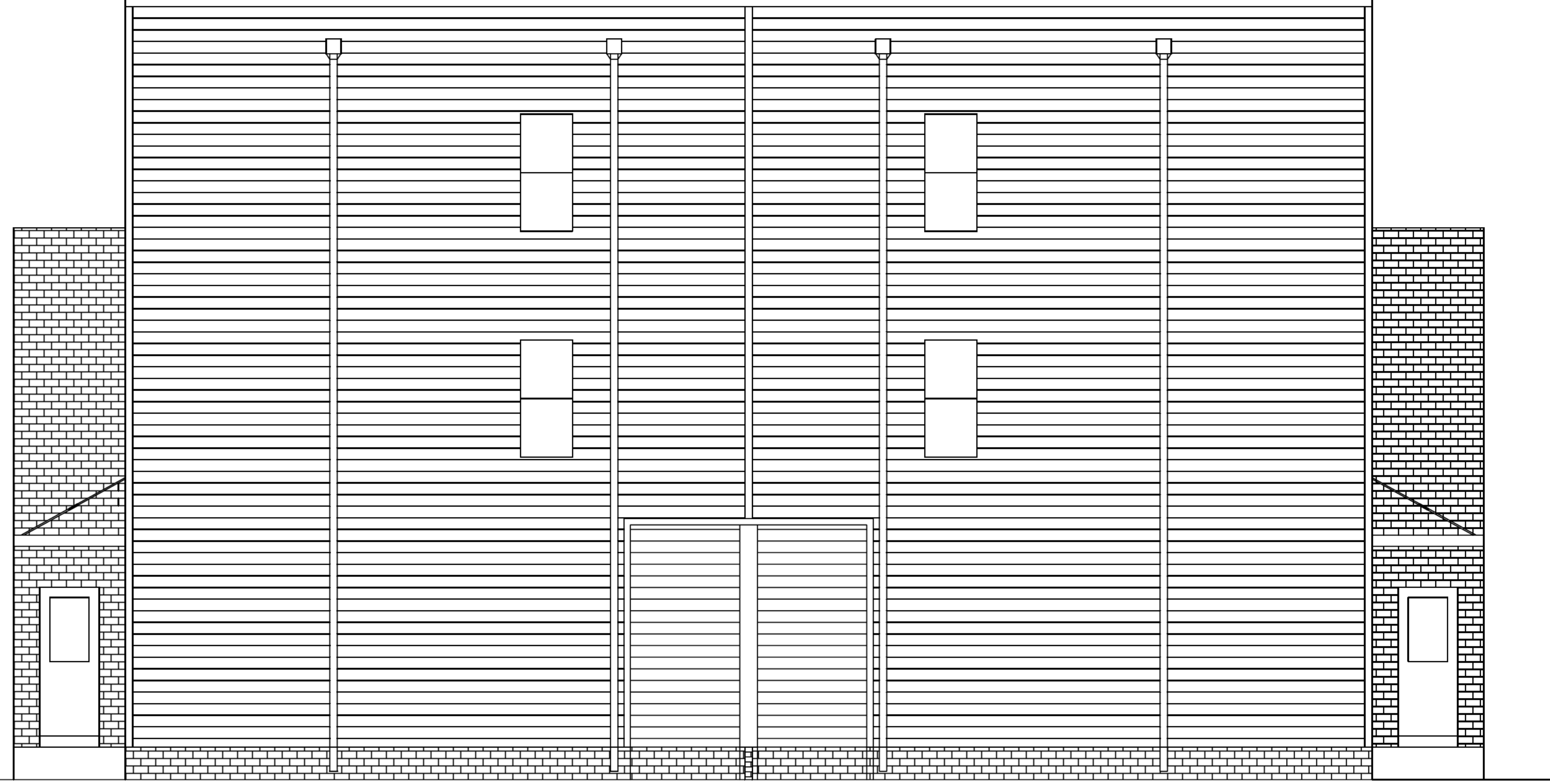
North Elevation 3/8" = 1'
