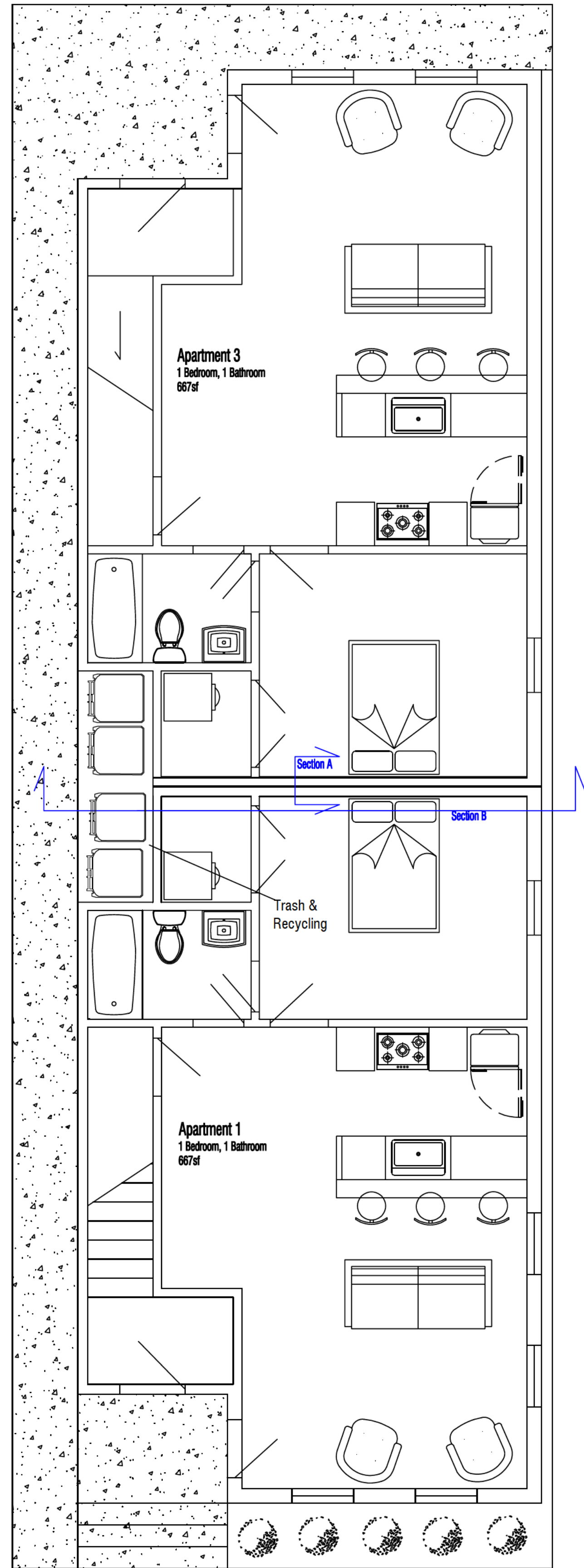
First Floor Plan 1/8" = 1'
