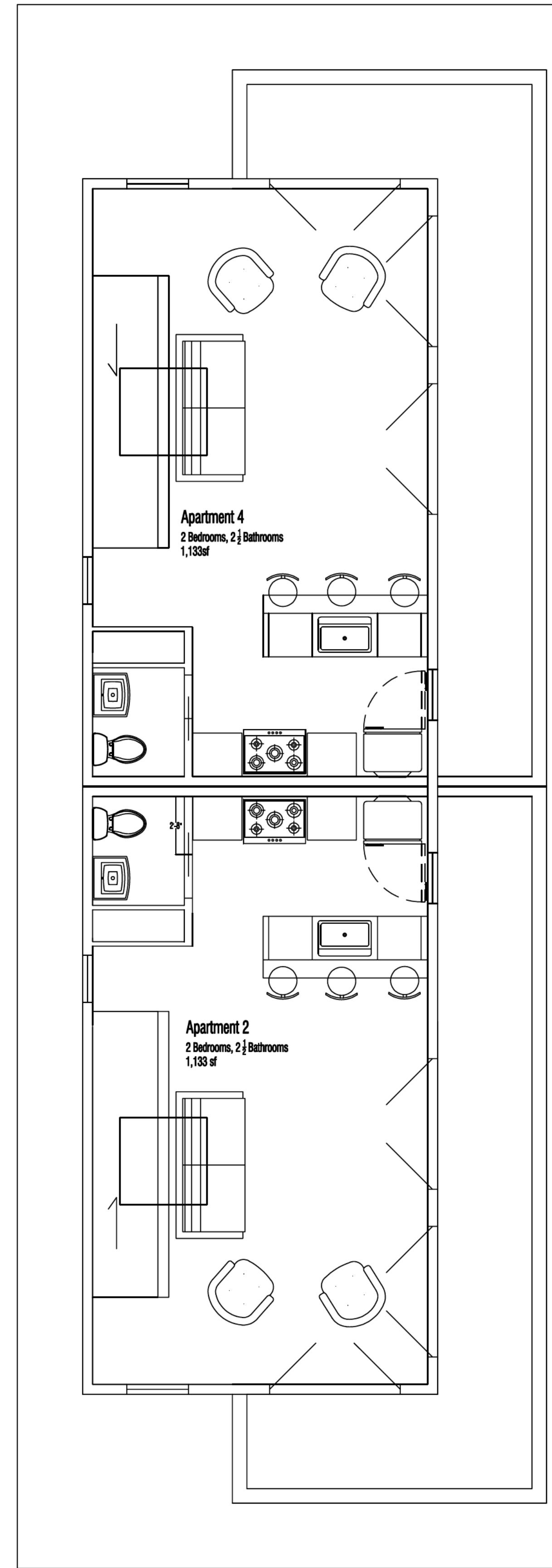
Third Floor Plan 1/8" = 1'
