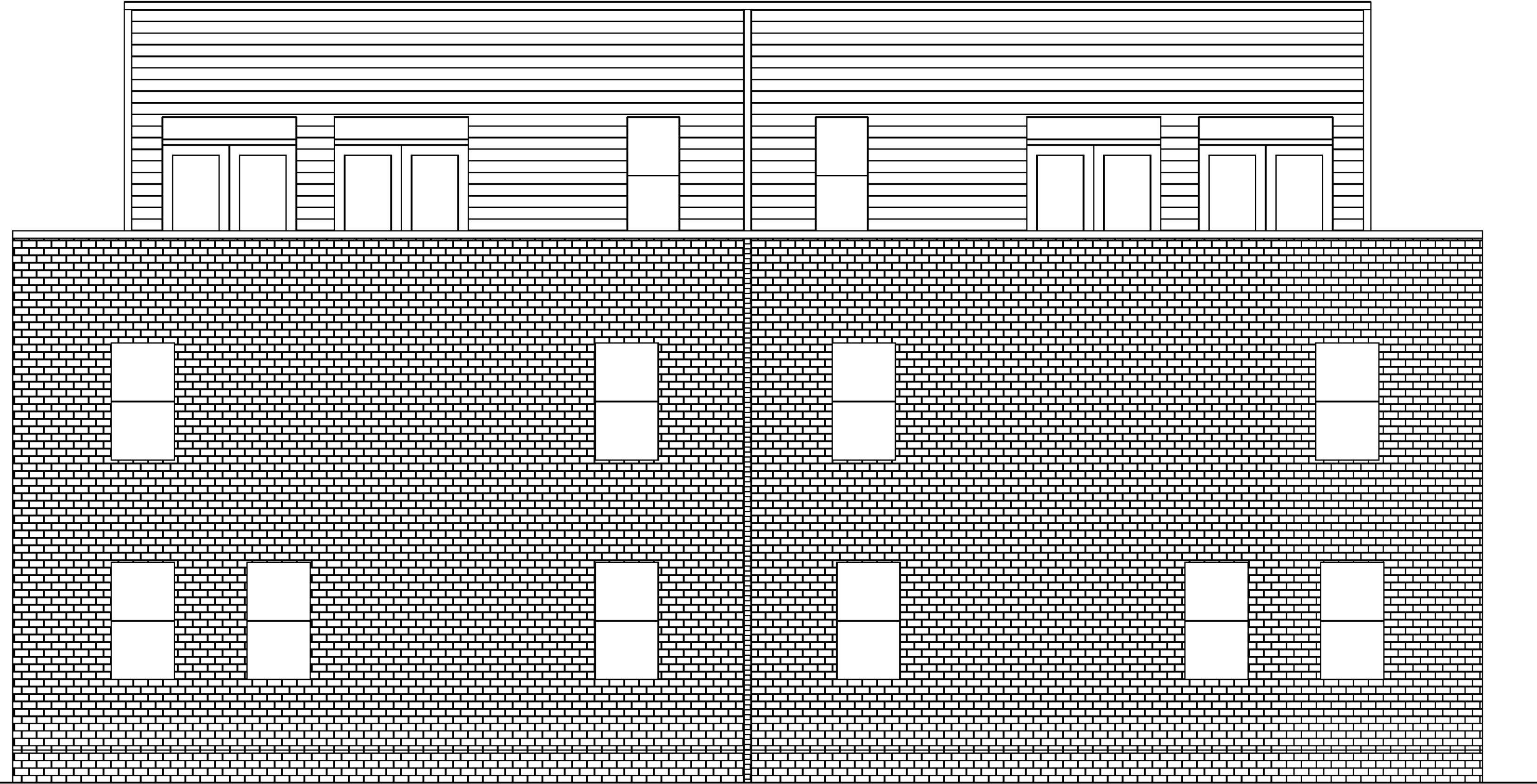
South Elevation 3/8" = 1'
