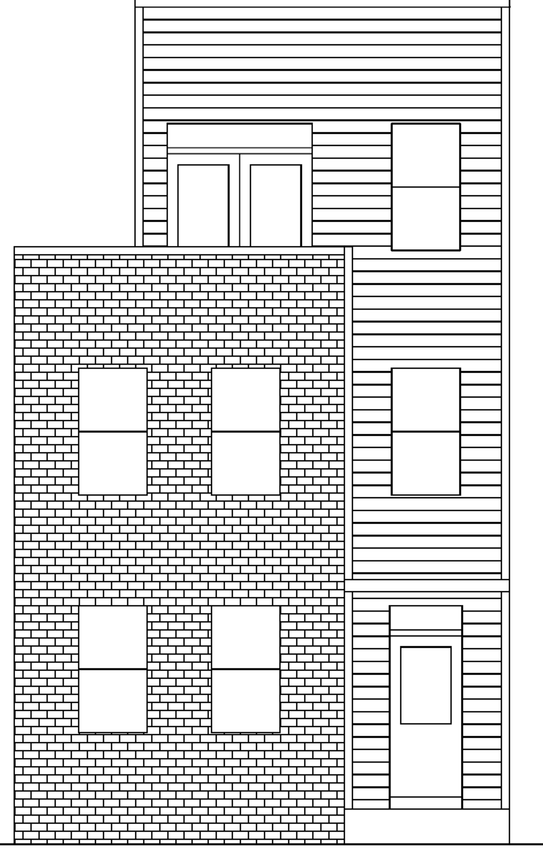
East Elevation 3/8" = 1'
