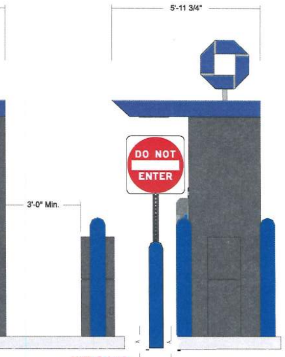
DEPARTURE ELEVATION
