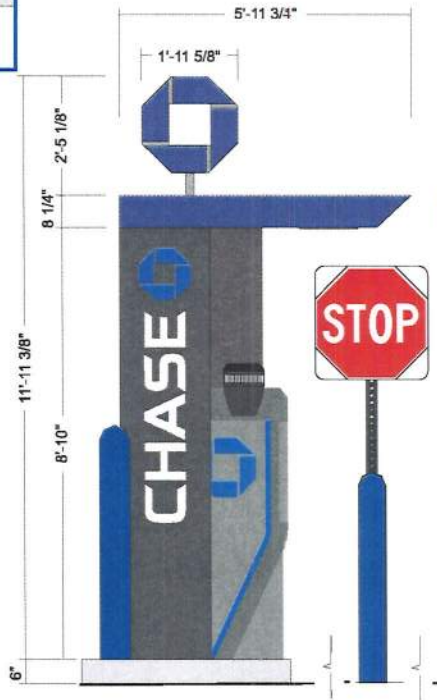
04 APPROACH ELEVATION
