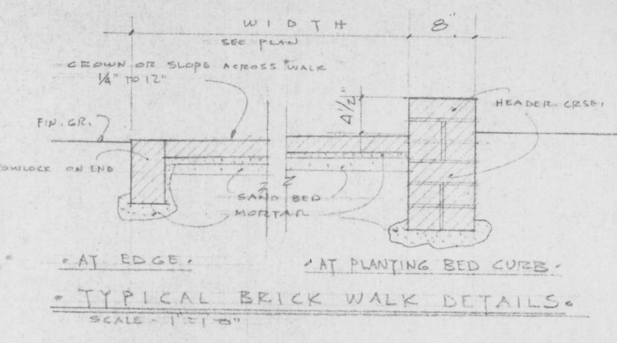
TYPICAL BRICK WALK DETAILS SCALE - 1" = 1'-0"
