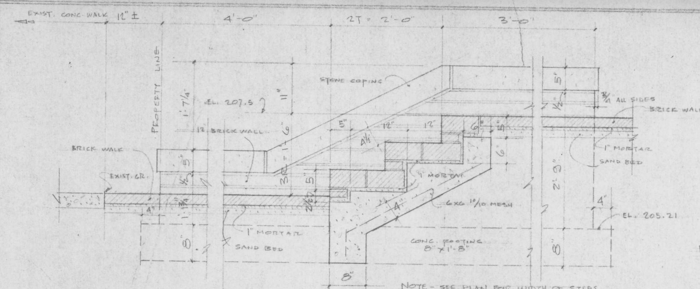
TYPICAL DETAIL - STEPS AT SIDEWALK SCALE - 1" = 1'-0"
