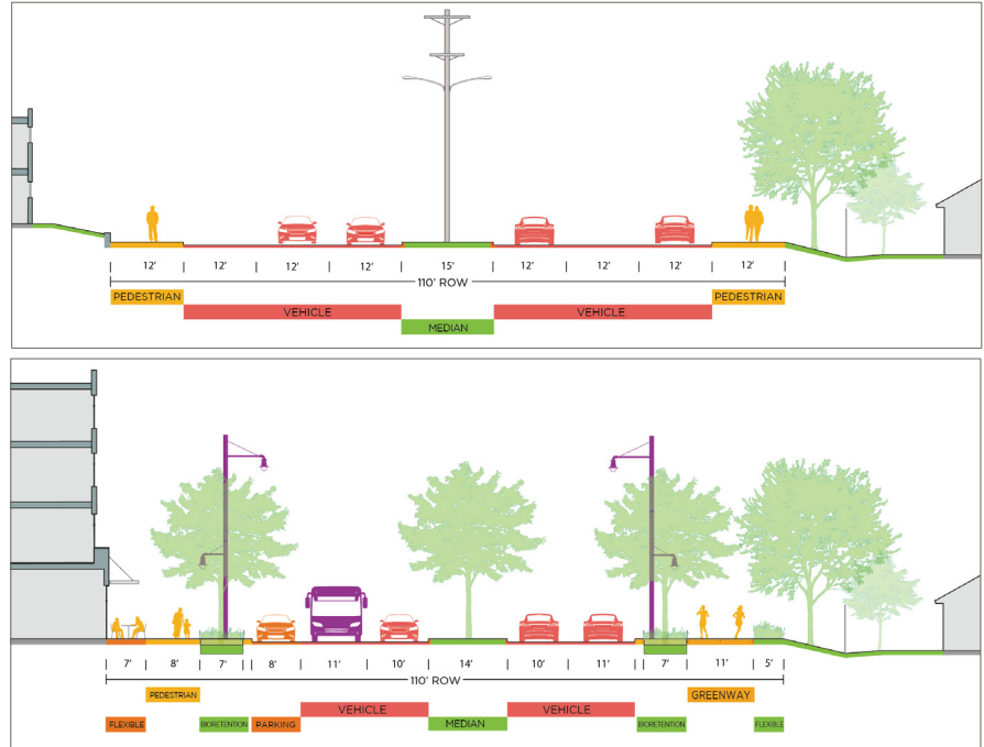
Route 1 Potential Street Section Transformation. The existing street [top] has more travel lanes than needed and can be transformed [bottom] into a complete street with elements such as outdoor seating, trees, pedestrian lighting, on-street parking, enhanced transit, car lanes, and a wide greenway (the Ashland to Petersburg Trail).
