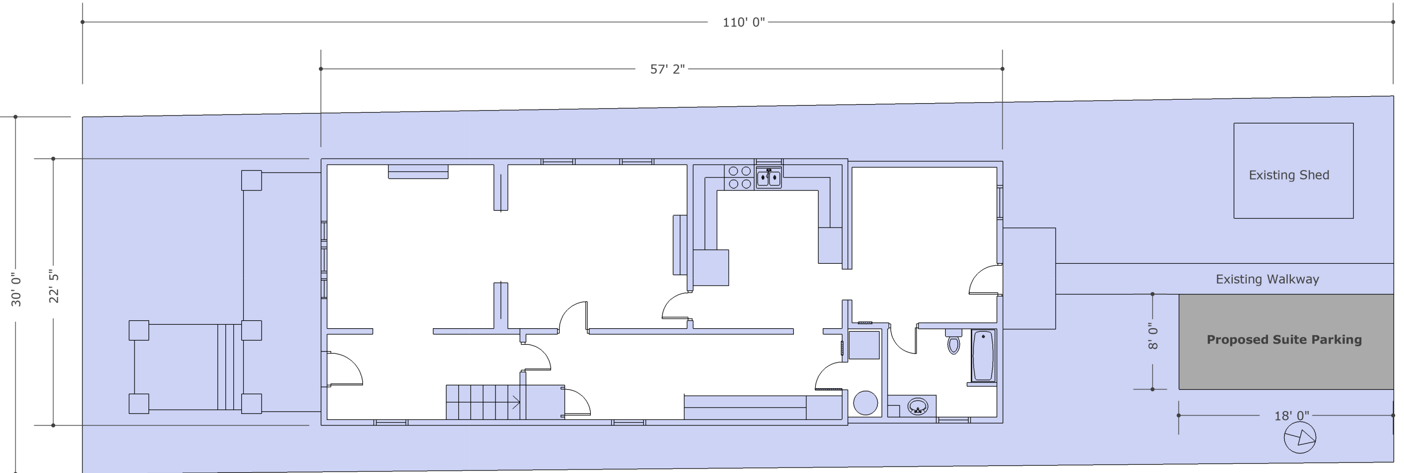
Existing first Floor Plan Shown On Lot
