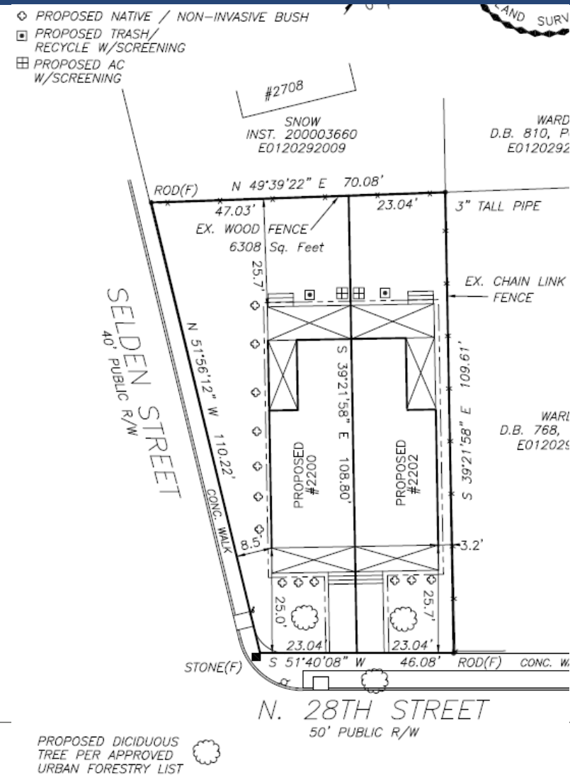
SITE PLAN
